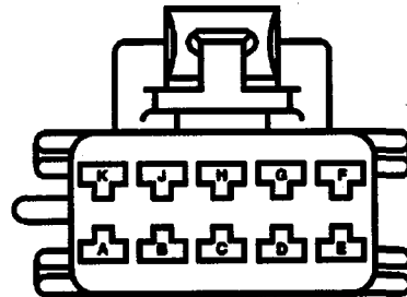
12064769 10-WAY F METRI-PACK 150 SERIES NAT SOLENOID VALVE ASSEMBLY (AQ9) PERFORMANCE SWITCH (PONT WITH M30 AND NW9) PERFORMANCE/TRACTION CONTROL SWITCH (PONT WITH M30 W/O NW9)
