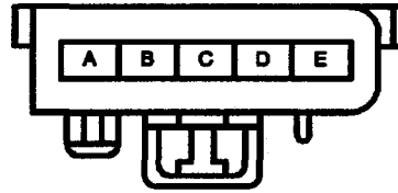
12059296 5-WAY F METRI-PACK 480 SERIES RED REAR DEFOGGER SWITCH/TIMER (CHEVY)
